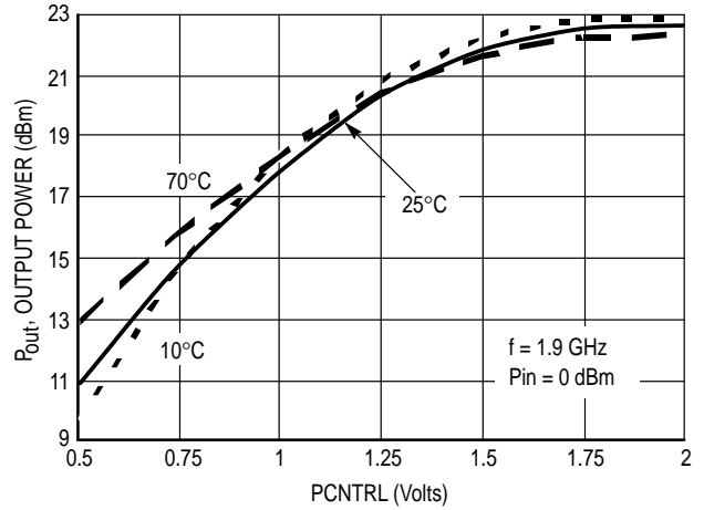
Figure 23. Pout versus PCNTRL Without Internal Logic Translator
